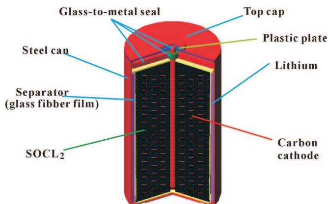
Bobbin construction
