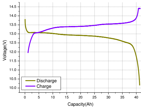
12.8V38.4Ah Charge-Discharge Curve 0.2C,25°C
