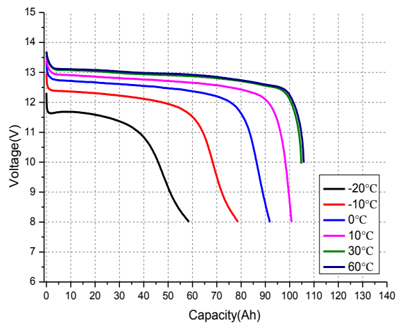
Discharge Curves at Different Temperature
